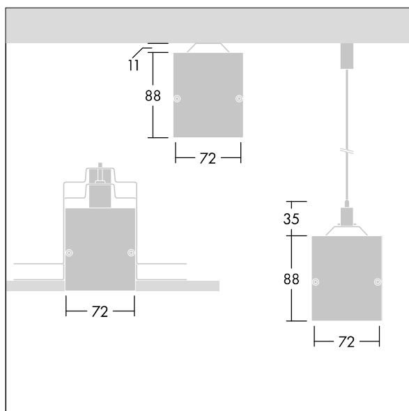
TLG_EQUL_M_surface_suspended_plasterboard.wmf
